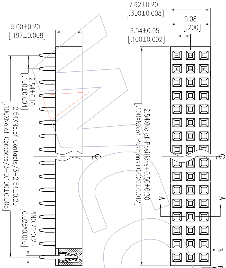
SECTION: B-B
